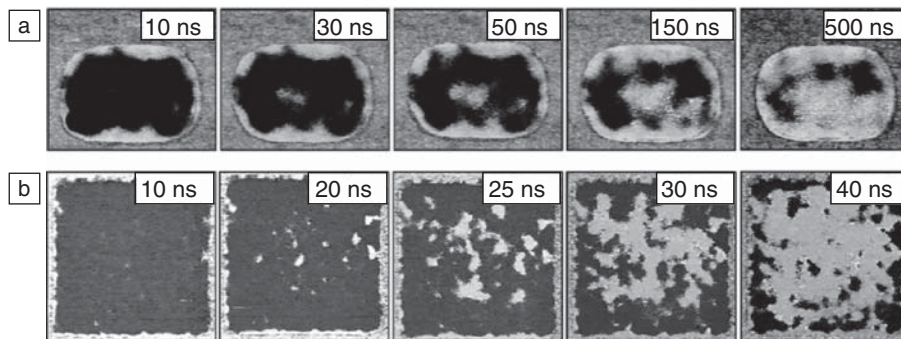
Figure 3. Piezoresponse force microscopy images of instantaneous domain configurations developing in (a) 1 \times 1.5 \mu\text{m}^2 and (b) 5 \times 5 \mu\text{m}^2 capacitors at different stages of the polarization reversal process for the same value of the applied field. The scanning area is 1.4 \times 1.8 \mu\text{m}^2 in (a) and 5 \times 5 \mu\text{m}^2 in (b). Reprinted with permission from Reference 14.
